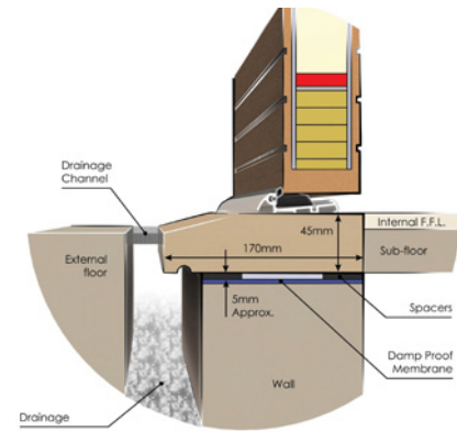
e80 cill section
