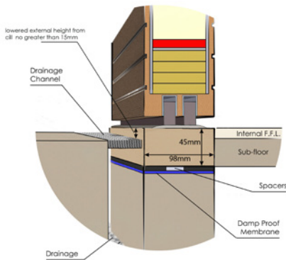
e98flush cill section
