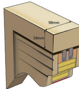
e98flush frame section
